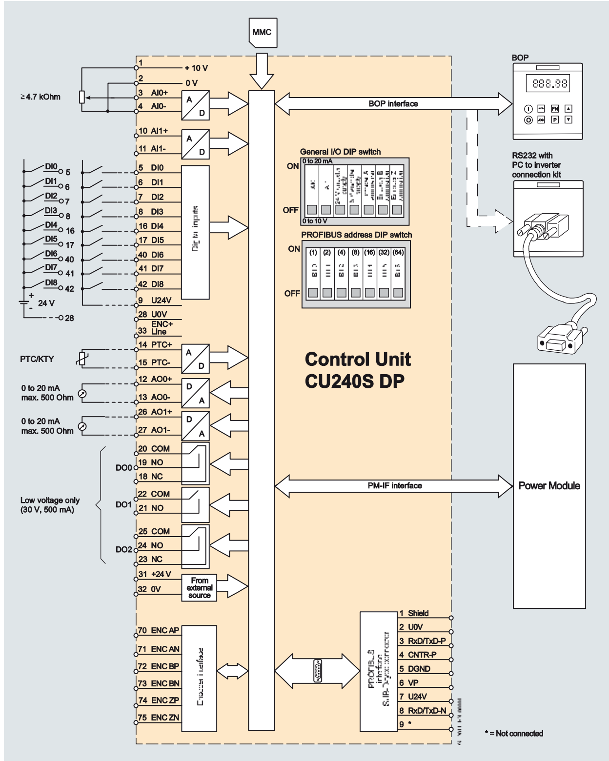
Connection diagram CU240S DP Control Unit
