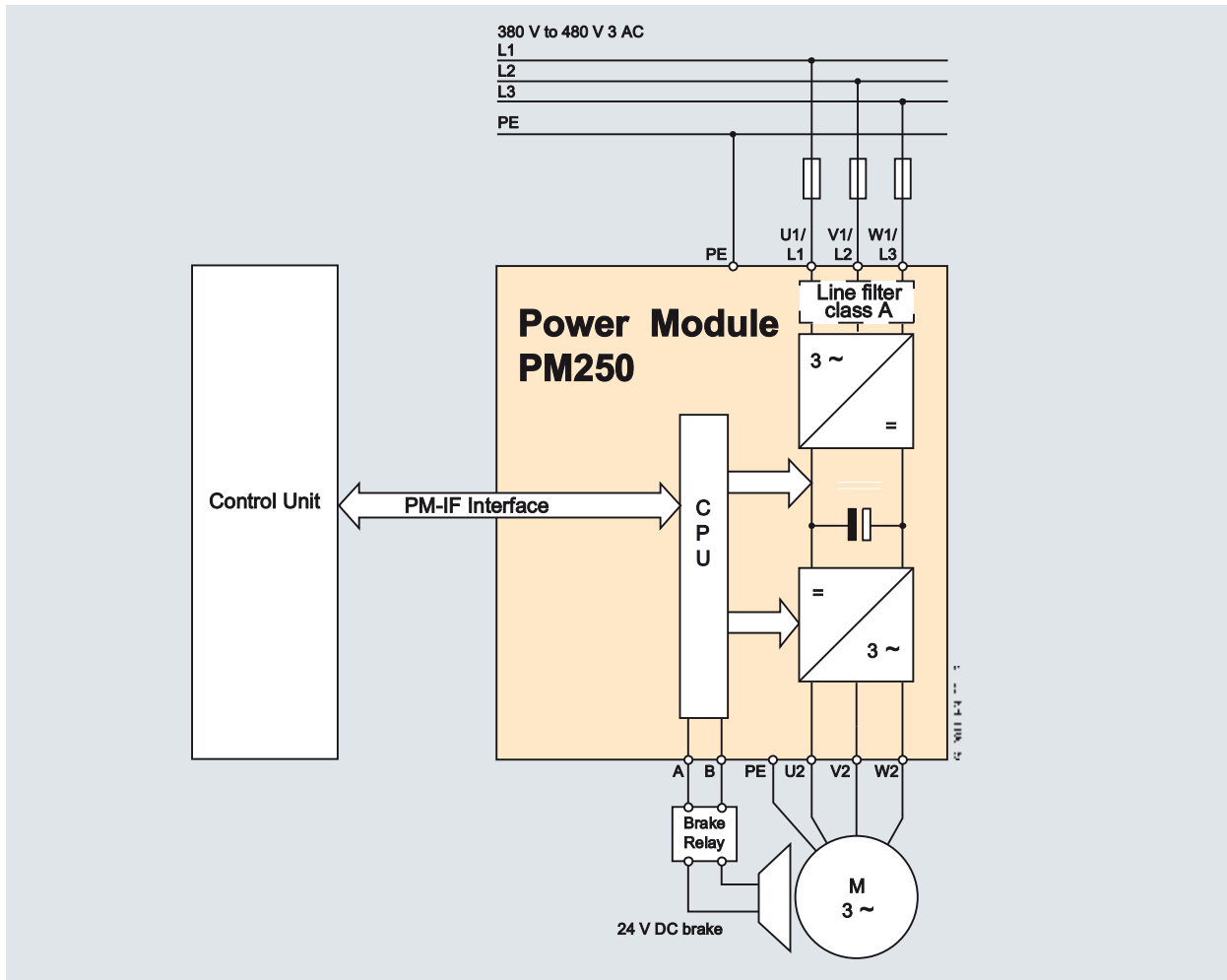
Connection diagram for PM250 Power Module with integrated line filter class A
